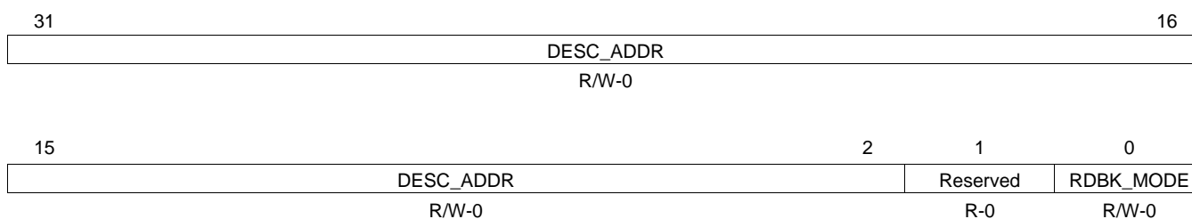
Figure 59. Receive CPPI Completion Pointer (RCPPICOMPTR)
